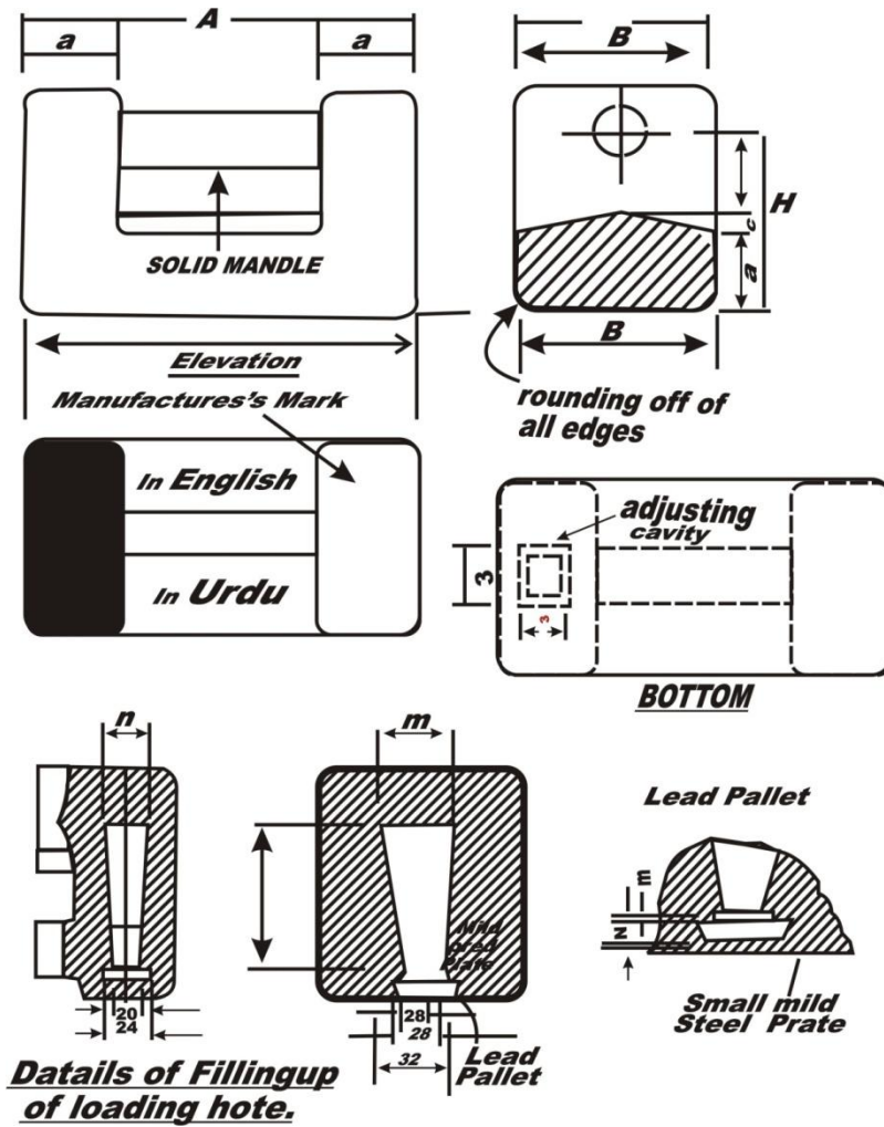
Fig – 2 Rectangular Bar weight with cast iron handle
