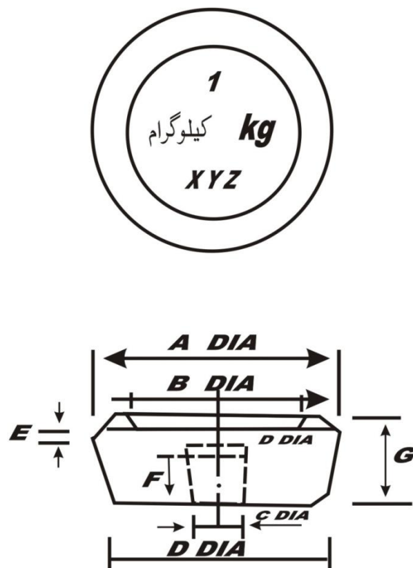
Fig 3. Flat Cylindrical Weight
