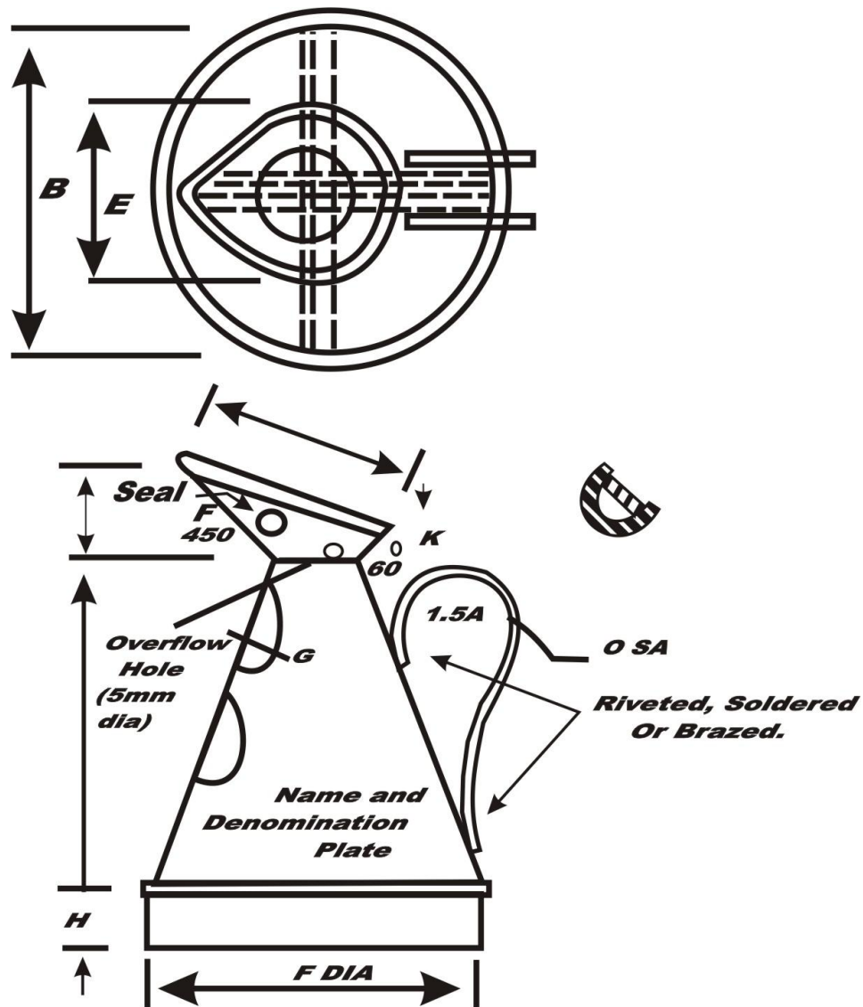
Fig. 2. Pouring Tote Conical Measure (Schematics)
